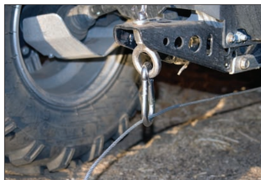
A strong stainless steel I-Bolt gets installed in the rear hitch mount to guide the winch cable. This piece also keeps the ATV from doing an endo on the very steep descents.
